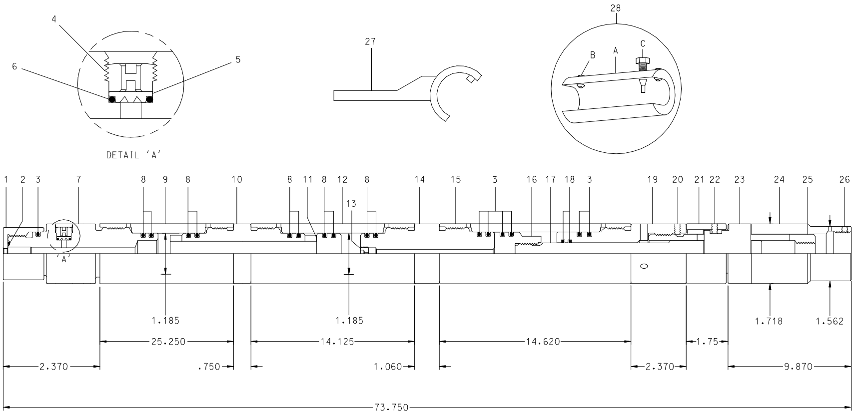
Figure 1: Assembly and Dimensional Data Drawing 390-979-00P02, Size 05
