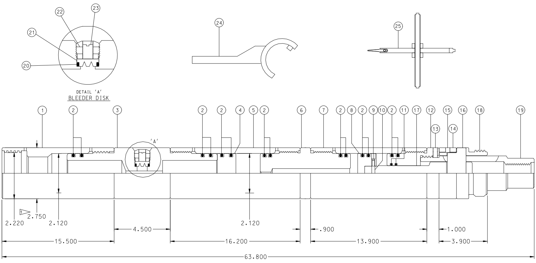
E-4 Wireline Pressure Setting Assembly Figure 2: Assembly Drawing 390-427-0P03, Size 10
