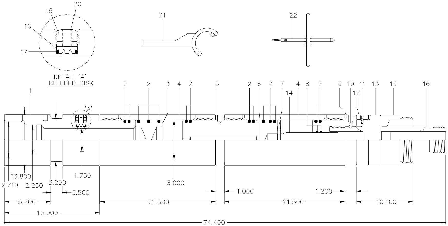
Figure 3: Assembly and Dimensional Drawing 390-426-00-3, Size 20
